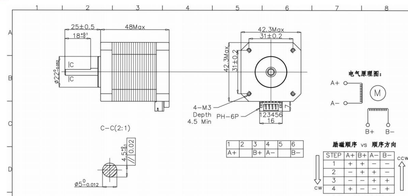
电机图纸 Motor drawings
