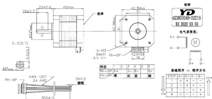
电机图纸 Motor drawings
